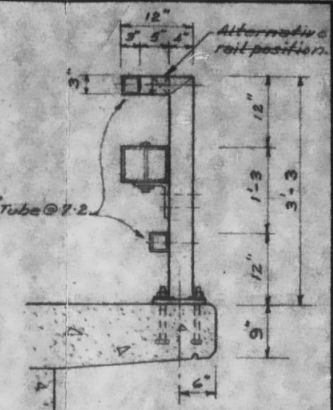
SIDEWALK scale \frac{3"}{4} = 1'-0"
