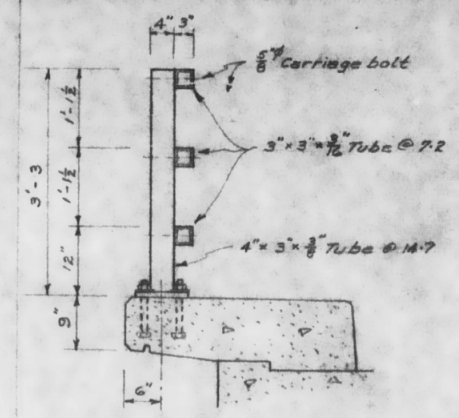
SAFETY CURB Scale \frac{3}{4}'' = 1'-0
