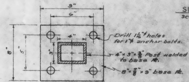
BASE PLATE Scale 3" = 1'-0"
