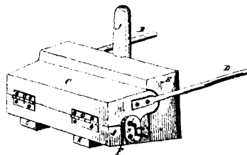
15264 Bradley's Improvements on O G Eaves Trough Machines.
