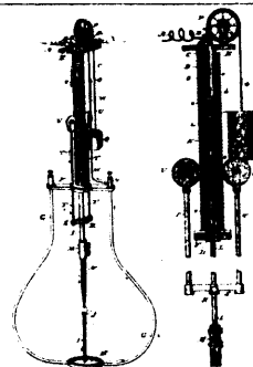
14458 Thomas & Skinner's Improvements on Electric Lamps.
