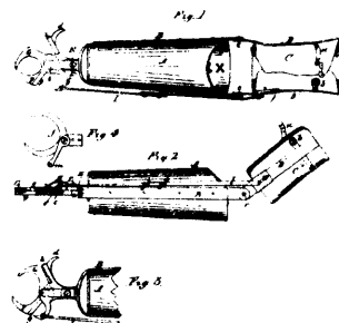
14455 Bowes's Improvements on Artificial Hands.
