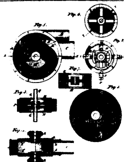
14470 Gurd's Improvements on Rotary Motors.
