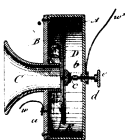
14454 Watson's Improvements in Telephones.
