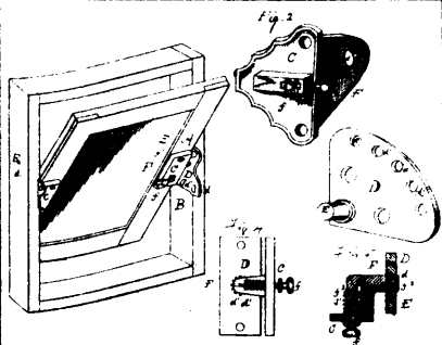
14459 Phillips's Improvements on Transom Pivots.
