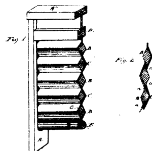
14464 Gates's Improvements on Wash Boards.
