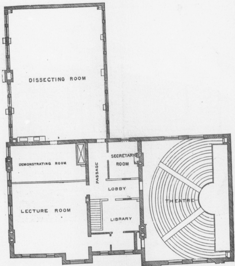
Plan—SECOND FLOOR.
