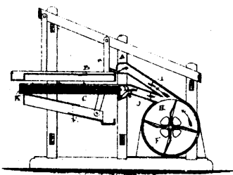
10220 Crone's Improvements on Threshing Machines.
