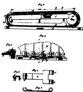
10223 Benjamin's Improvements on Horse Powers.
