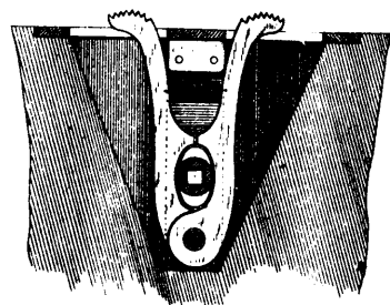
10216 Teagley's Improvements on Sash-Holders.
