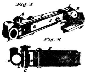
10214 Bradley's Improvements on Harvester Pitmans.
