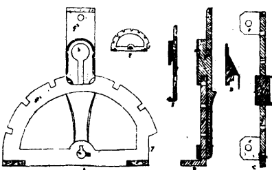
9329 Robinson's Hinge for Attaching Buggy Tops.
