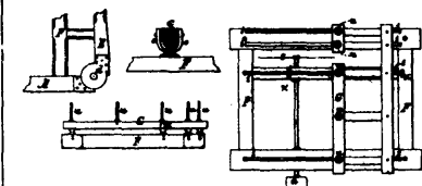
18199 Dunckel's Portable Steam Sawing Machine.
