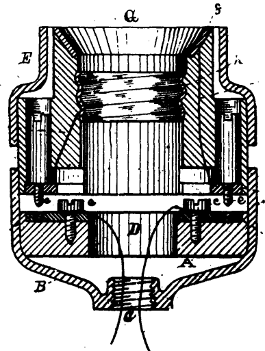
16095 Johnson's Improvements on Sockets for Electric Lamps.
