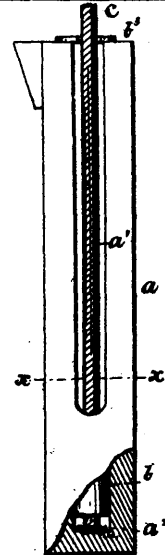
16103 Goforth's Improvements on Sash Cord Fasteners.
