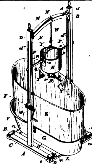
16101 Kendall's Improvements on Portable Bathing Apparatus.
