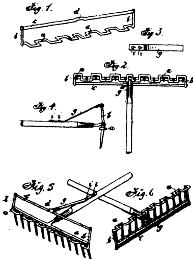
16097 Miller &amp; Eason's Improvement in Hand Rakes.
