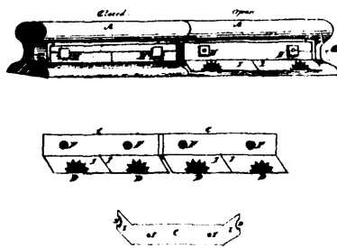
12706 Smith's Improvements on Nut Locks.
