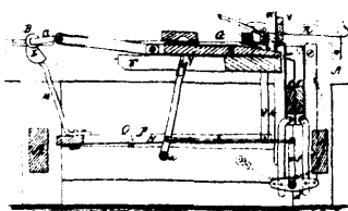
12711 Bidwell's Improvements on Shingle Machines.
