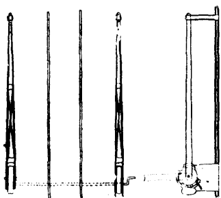
12705 Emond's Improvements on Gates for Railway Crossings.
