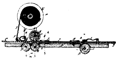
12702 Ripson's Improvements on Machines for Covering Moldings with Cloth.
