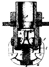
12701 Heylman's Improvements on Feed Water Heaters.
