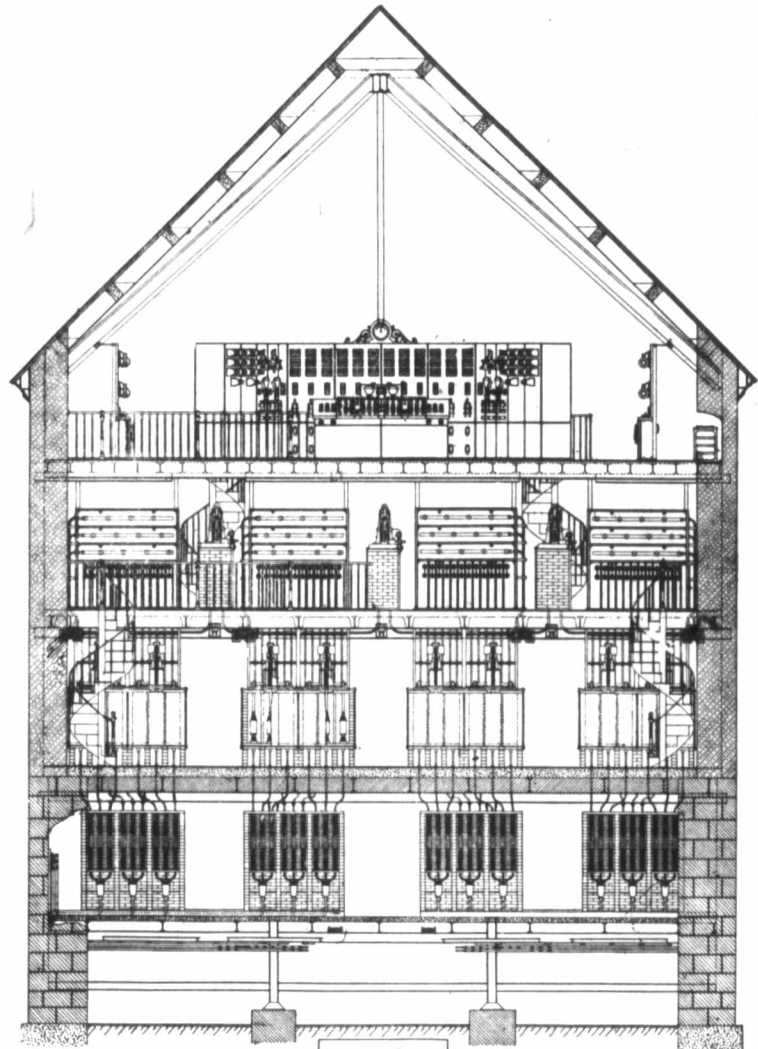
LONGITUDINAL SECTION GENERAL ASSEMBLY FROM EAST END AS SHOWN E 4
