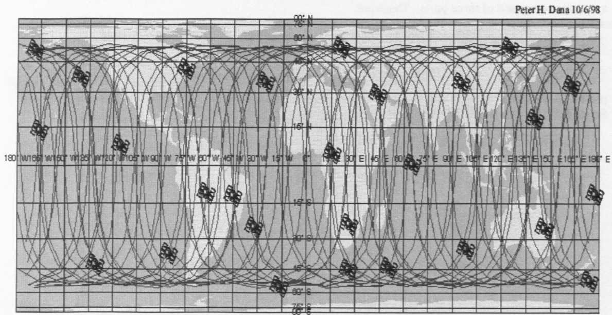
Global Positioning System Satellites and Orbits for 27 Operational Satellites on September 29, 1998
