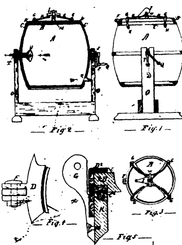
Smith & Kingleyside's Churn.
