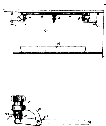
Stanford's Aerator for Wort.
