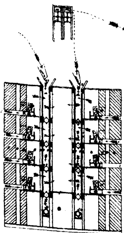
Borland's Kiln for Drying Grain.
