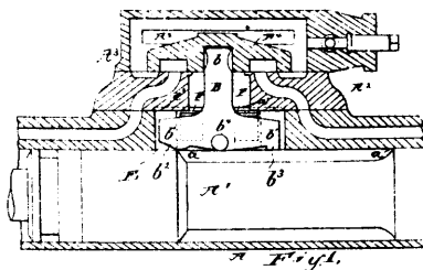
Rand's Rock Drill.
