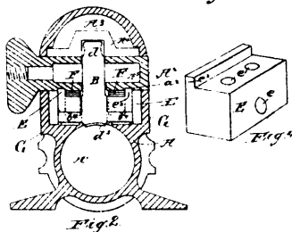
Githens' Rock Drill.
