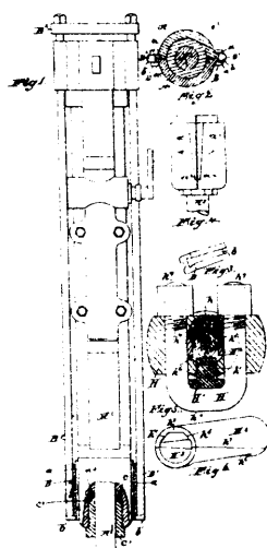
Rand's Rock Drill.
