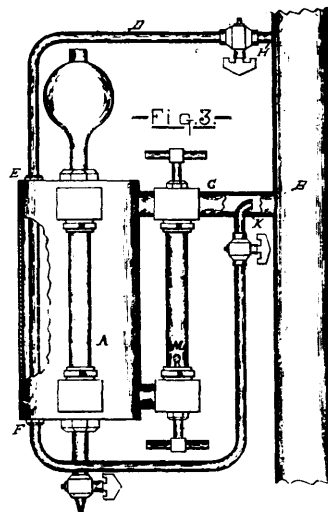
Green's Lubricator.
