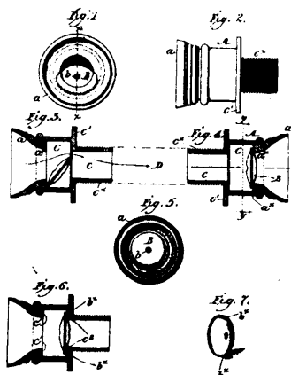
Green's Lubricator.
