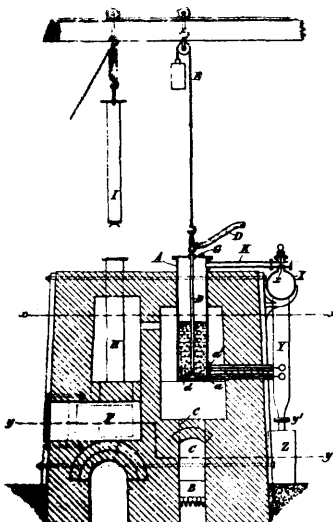
Beilby's Apparatus for Manufacturing Cyanides.
