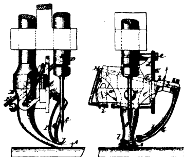
3187 Rose's Embroidering Attachment for Sewing Machines.
