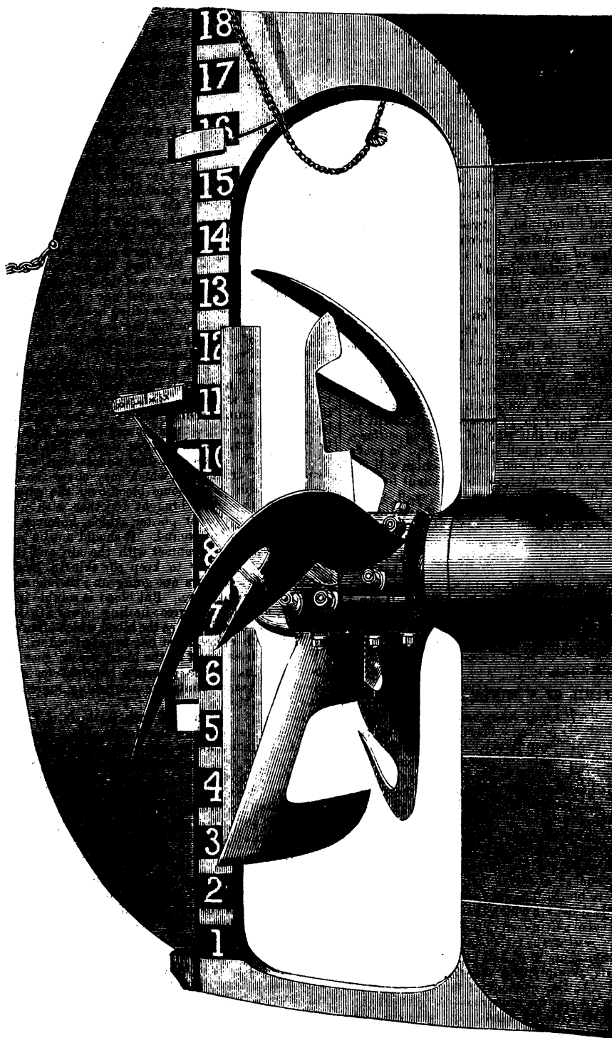
THE DE BAY PROPELLOR.—THE TWO HUBS WITH THEIR BLADES MOVE IN CONTRARY DIRECTIONS.
