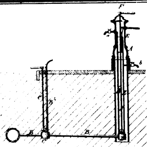
5628 Rapp's Improvement on Hydrants.
