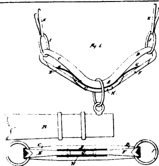
5634 Hickox's Improvement on Breast Irons.
