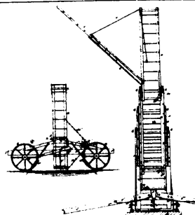
5631 Sandford's Combined Fireman's Ladder and Fire-escape.
