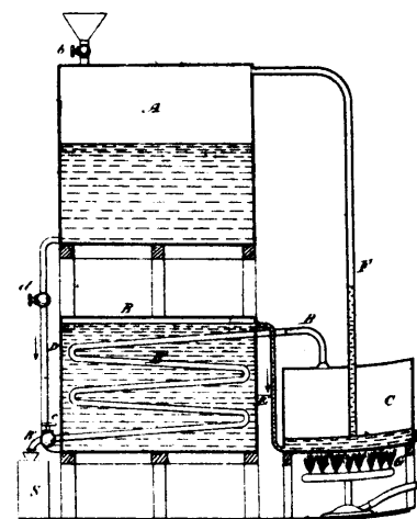
20034 Herrick's Apparatus for Distilling Water, &amp;c.
