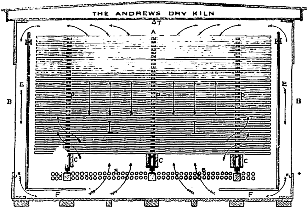
This system and apparatus covered by letters patent. A—Drying-Room. BB—Brass Condensing-Walls. CCO—Lumber Cars. EE—Down Air-Flues. FF—Bottom Air-Flue. HH—Inside Walls, protecting metal from heat. LL—Lumber on cars. NN—Brass Gutters for receiving condensed moisture. PPP—Sticks between lumber. SS—Double Steam-Coils. T—Automatic Steam Fire-Extinguishers. Arrows show direction of currents of air.
