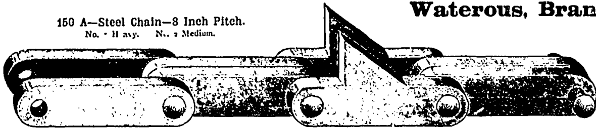
No. 105—Special Heavy Chain, 6" Pitch. Made in Sizes. Showing Coupler and Forged Log Spur.
