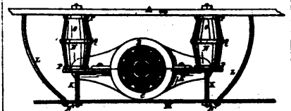
7900 Wilcox & Kelsey's Railway Journal Box.
