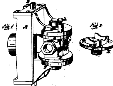
7899 Flower's Chuck for Holding Pipe Fittings.
