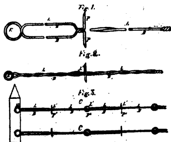
7911 Crandal's Improvements on Barbed Wire Fences.
