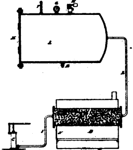
7902 Robbins' Process of Seasoning and Preserving Wood.
