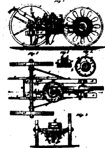
7814 Custer's Combined Potato and Corn Planter.
