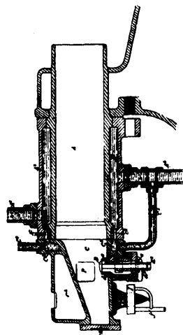
40096 Pinkney's Gas Engine.
