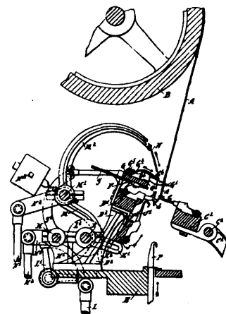
40093 Stuart's Machinery for Making Nets
