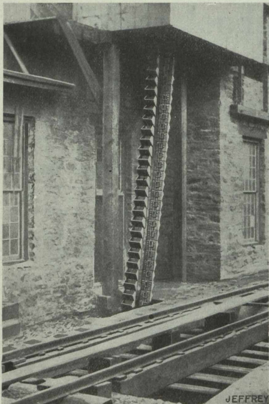
Jeffrey Bucket Elevator handling Ore from Track Hopper to Bin, Northwestern Metals Co., Helena, Montana.
