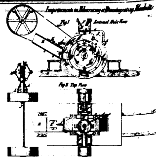
7089 Lipsey's Improvements on Pulverizing Machines.
