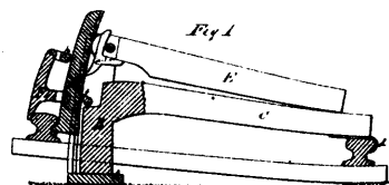
7096 Hunter's Lifting Jack for Railroad Tracks.
