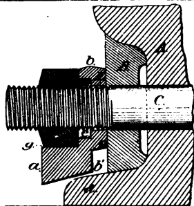
7098 Latham's Improvements on Nut Locks.
