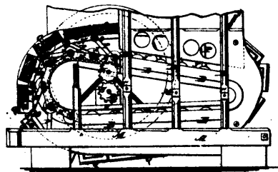
7090 Trulender &amp; Warburton's Improvements on Horse Power.
