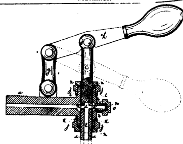
7092 Andrews &amp; Hutchinson's Improvements on a Guage Cock.
