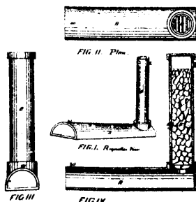
7101 Hicks &amp; Tracy's Improvements in Gas Meters.
