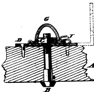
7091 Carpenter's Improvements in Nut Locks.
