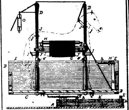
36743 Sample's Apparatus for Taming Horses.
