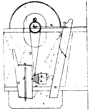
36743 Sample's Apparatus for Taming Horses.
