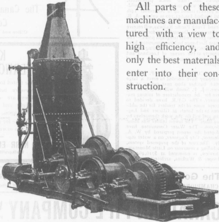
Double Cylinder, Double Drum Hoisting Engine with Swinger.
