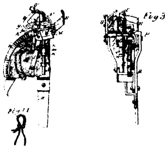
11936 Storle's Improvements on Grain Binders.
