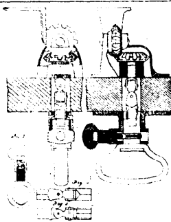
11938 Troy's Improvements on Blind Hinges.
