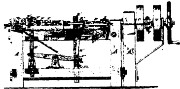
9629 Jones's Improvements on Machines for Manufacturing Tobacco.
