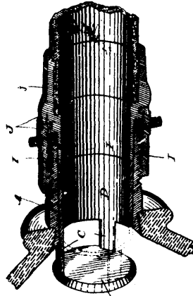
35074 Redican's Hydrant.
