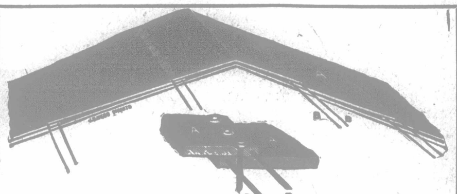
A shows method of laying Red Star Brand Wire-edged Ready Roofing, with 2-inch laps secured by nailing two inches apart. B B shows wires running through the edges of the roofing, giving it great strength at the joints or laps—a very desirable feature, especially in localities where high winds prevail.
