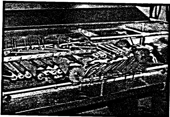
View of feed trays and head cutting apparatus on 'Simor' Automatic Heading/Eviscerating Machine.
