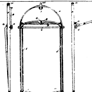
2483 Ludiam's Harpoon Fork.
