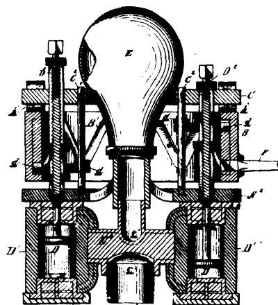
20241 Halsey's Horse Power Fire Engine.
