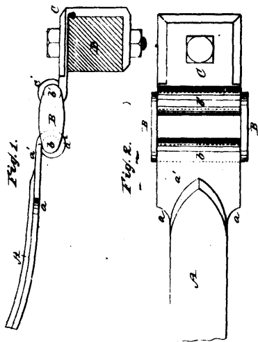
20236 Marshall's Side Spring Carriage.
