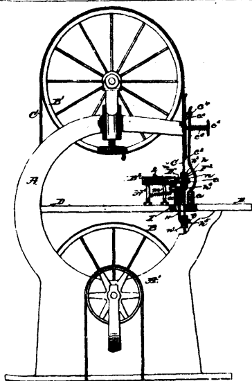
20239 Campbell's Machine for Preparing Hoops.
