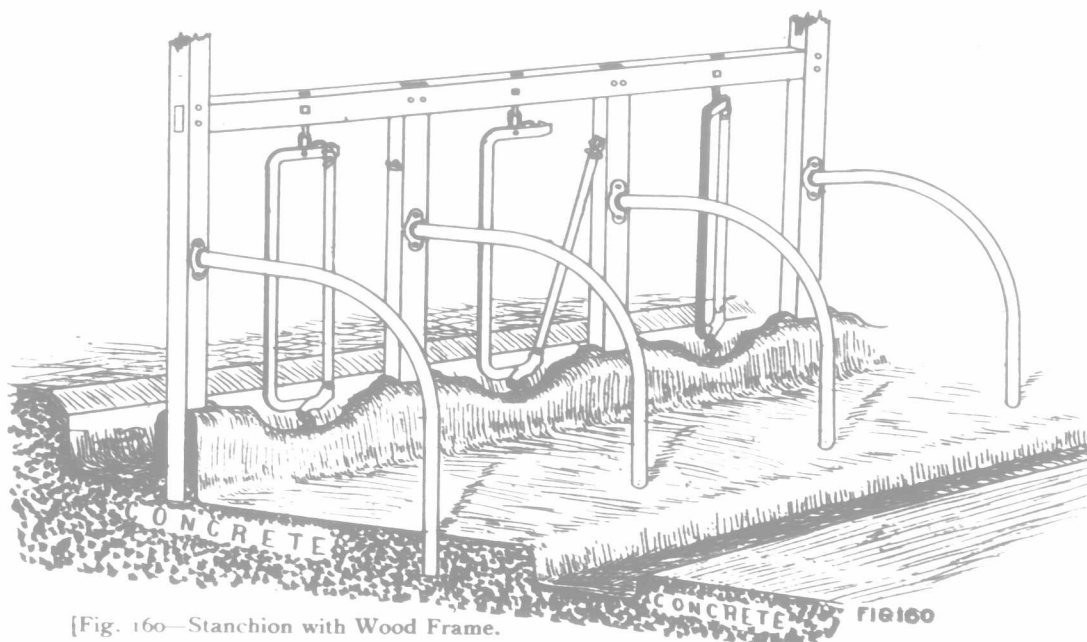
[Fig. 160—Stanchion with Wood Frame.]
