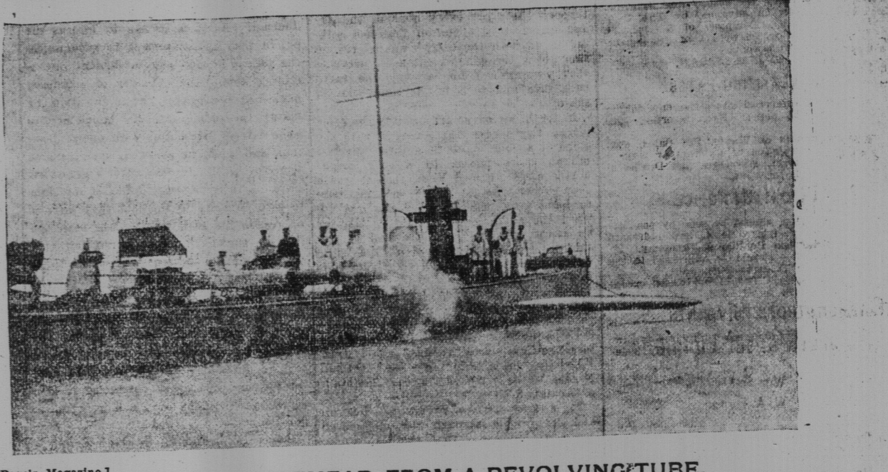
FIRING A WHITEHEAD FROM A REVOLVING TUBE.
