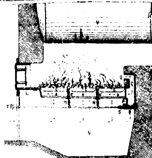
12381 Nitsche & Grellmuth's Improvements on "Fire-place" for Steam Boilers.
