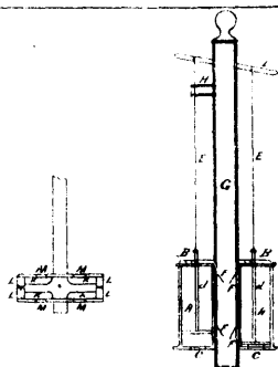
12369 Bickford's Improvements on Force Pumps.
