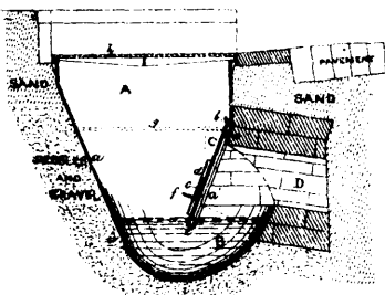
2774 Dark's Receiver and Stench Trap of Street Sewer.
