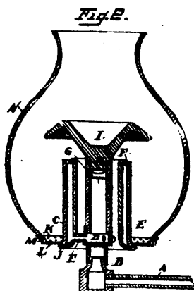
Morey's Gas Burner.
