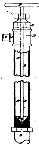
33963 Houlgrave's Steam Trap.
