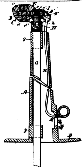
18950 Wakefield's Machine for Cutting Pegs from Boots and Shoes.
