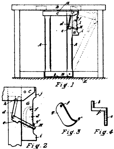
18948 Smith's Stanchion for Cattle.
