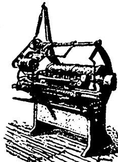
COMBINED SPOKE TURNING AND SQUARING MACHINE. Capacity, 2,500 Spokes per day.
