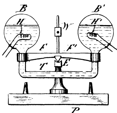
30803 Thomson's Electro Mechanical Movement.
