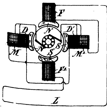
30802 Thomson's Electric Machine.
