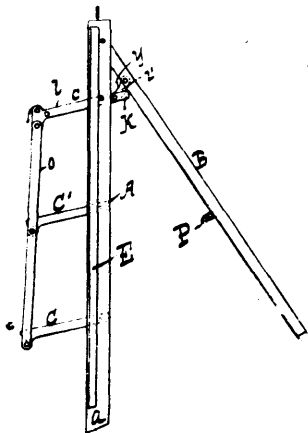
30797 Dormitzer's Step Ladder.
