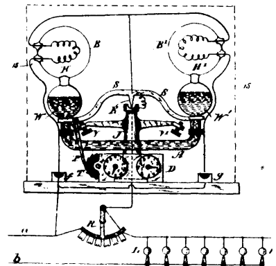
30804 Thomson's Electric Meter.
