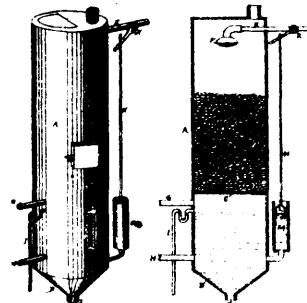
13194 Dane's Improvements in Apparatus for Purifying Feed Water for Steam Generators.
