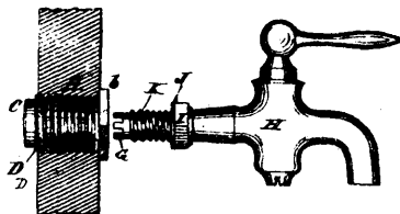
13196 Gaines's Improvements on Faucet Bushings and Faucets Combined.
