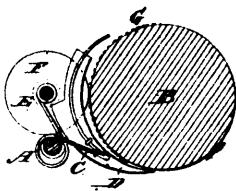
13182 Pratt's Improvements on Paper Pressers for Type Writing Machines.
