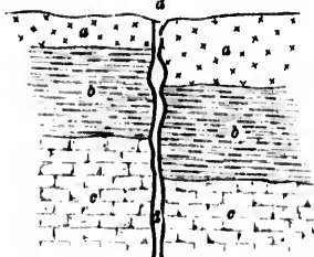
SECTION OF A VERTICAL FAULT.
