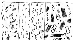
a, ZONE OF LARGER CRYSTALS OF MICA AND HORNSLENDE. b, APATITE AND HORNSLENDE. c, CHIEFLY HORNSLENDE. d, MICA ROCK.
