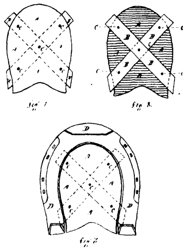
15850 Marshall's Improvement in Horse Shoes.
