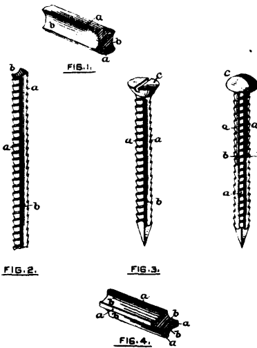
15849 Rogers' Improvements on Screw Nails.
