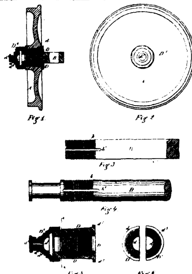
15857 Fairman's Improvement in Car Wheels and Journal Bearings.
