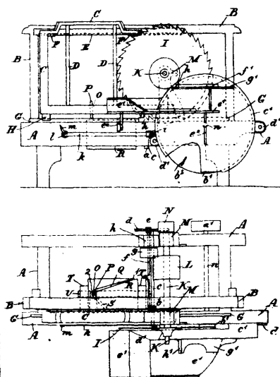
15856 Frechette's Improvements in Shingle Machines.
