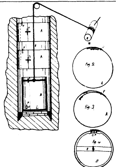
15855 Davis' Improvements in Devices for Digging and Lining Wells with Cement.
