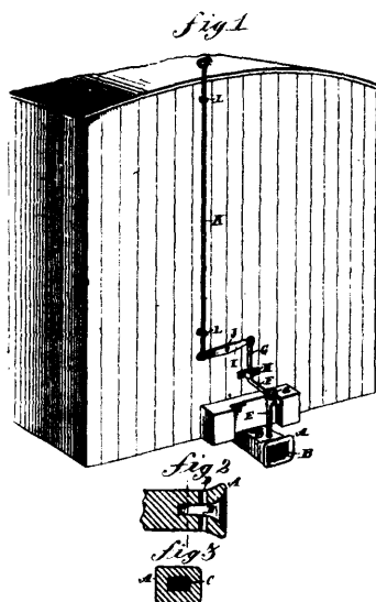
15853 Brown's Improvements on Car-Couplings.
