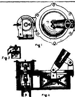
7362 Ellis &amp; Loud's Improvement on Ships' Pumps.
