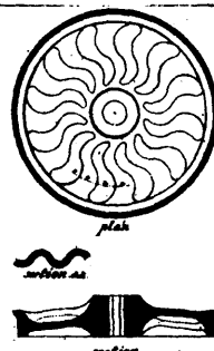
7366 Urquhart's Improvements on Car Wheels.
