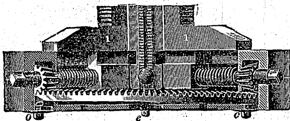
Fig. 2—Circular Chuck.
