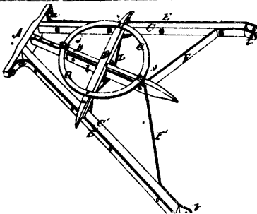
8038 Fitch &amp; Roth's Improvements on Waggon-Trestles.
