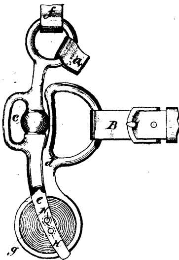
Chandler's Bridle Bit.
