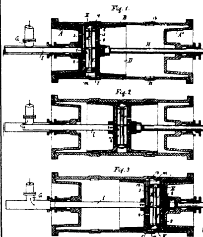
30931 Laun's Motor.
