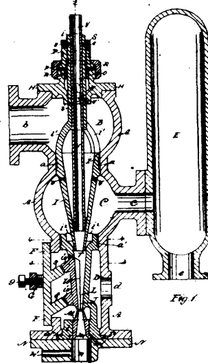
30932 Killey's Injector.
