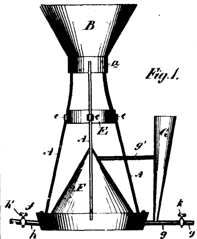
30930 Macpherson's Milk Purifier.
